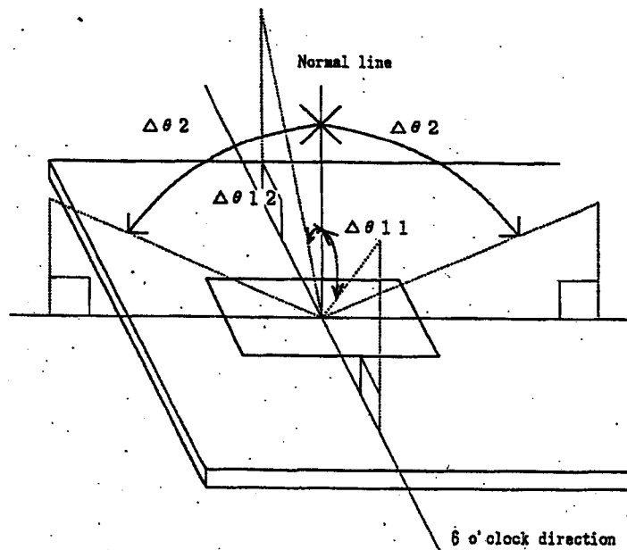
Fig. (i) Definition of viewing angle
