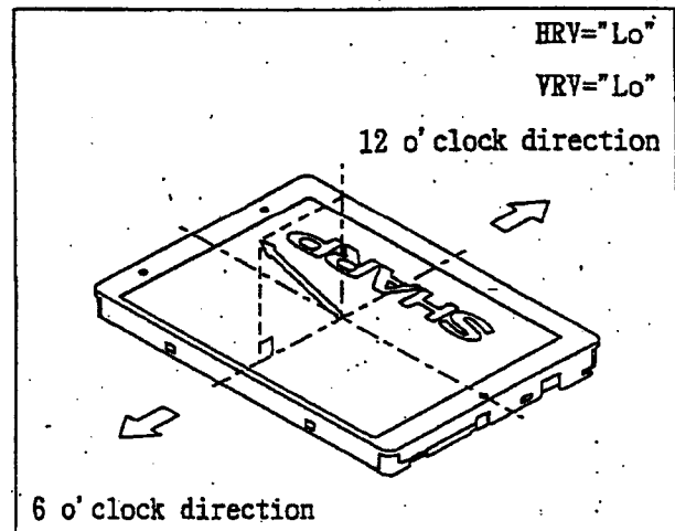
Fig. E. 12 o'clock direction type
