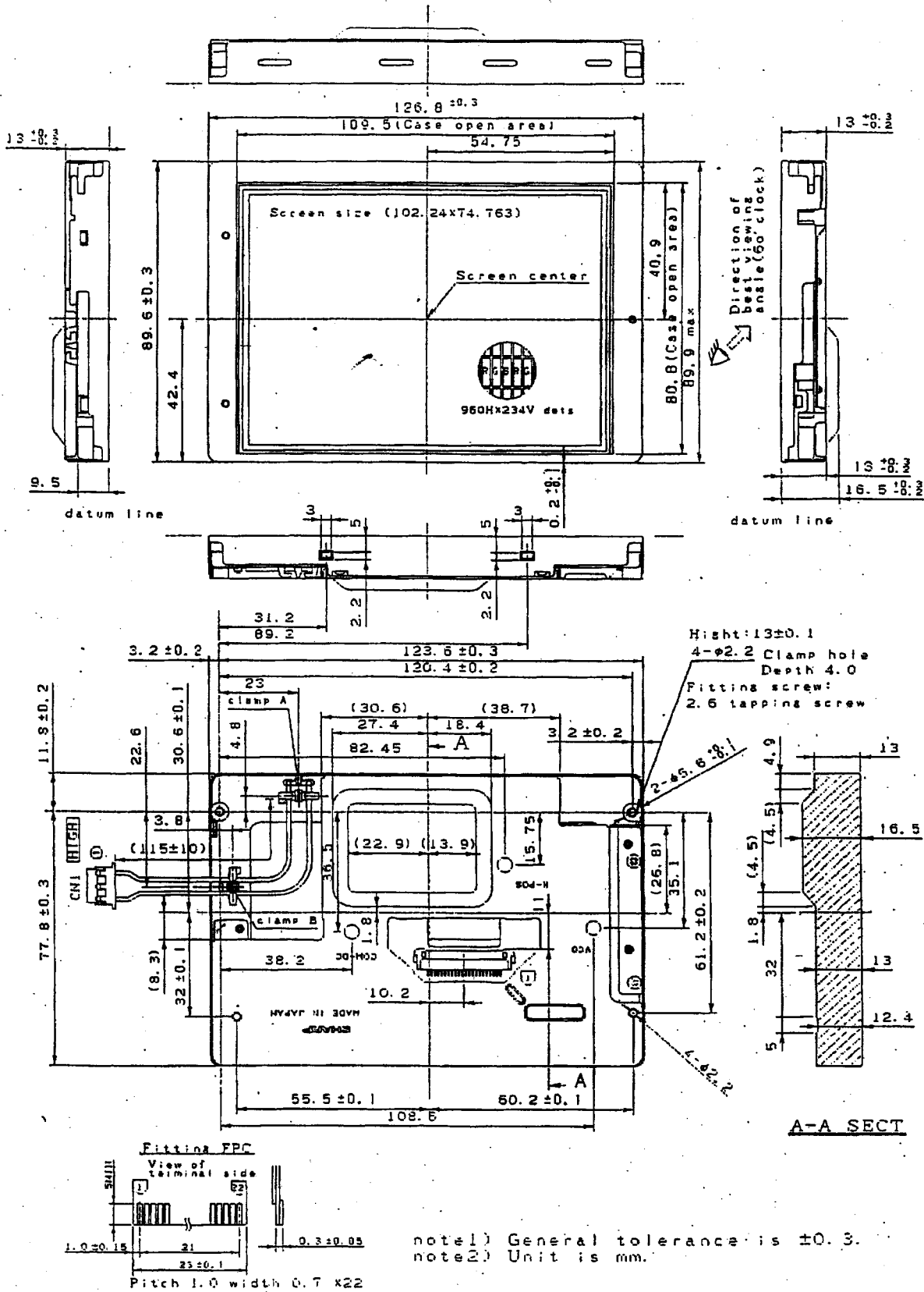
Fig 3. Outline dimensions of TFT-LCD module
