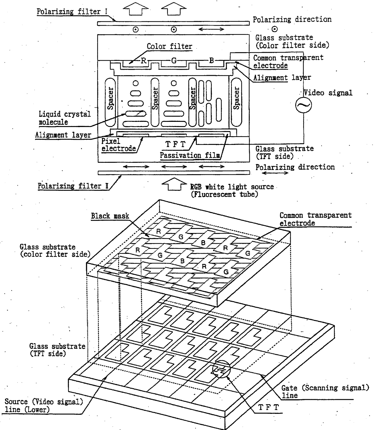
Fig 1. Illustration of TFT-LCD panel
